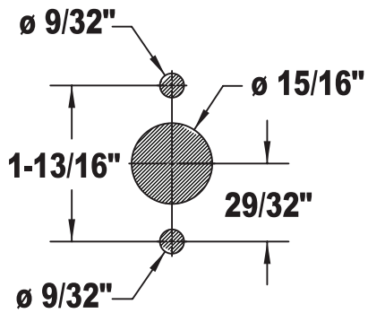
MOUNTING HOLES
