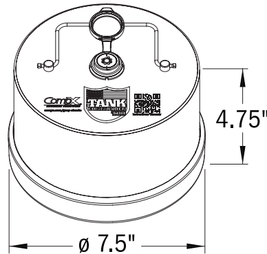
Turbine TANK Commander Too (P/N: TCT-2)
