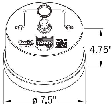
TANK Commander Too without padlock (P/N: TCT-PL-NL)
